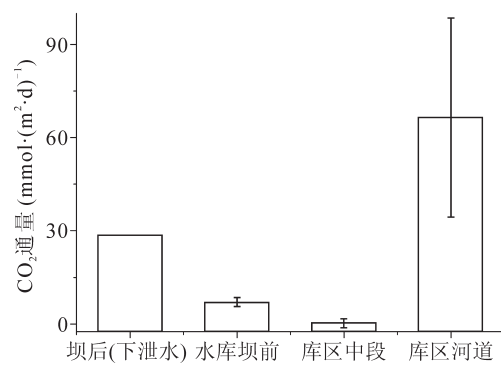
图6 新安江一千岛湖水库各段 CO 2 释放通量 Fig.6 Release flux of CO 2 in different parts Xin'anjiang-qiandao lake reservoir
