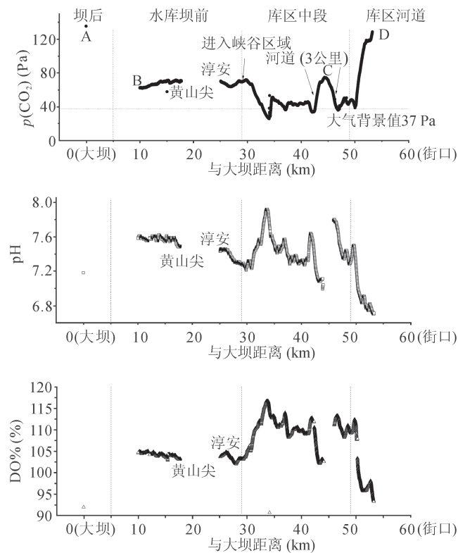
图 2 新安江—千岛湖水库走航观测结果 Fig.2 Result of continuous measurement in Xin'anjiang-qiandao lake reservoir
